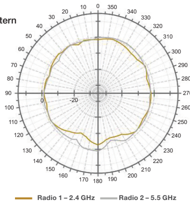
E-Plane Pattern
