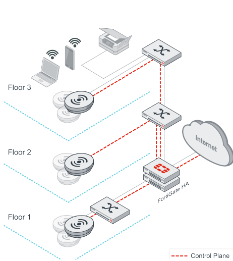
A central pair of FortiGates managing a large site
