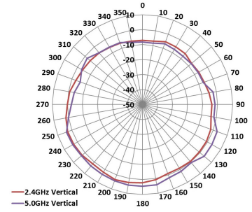
E-Plane Pattern
