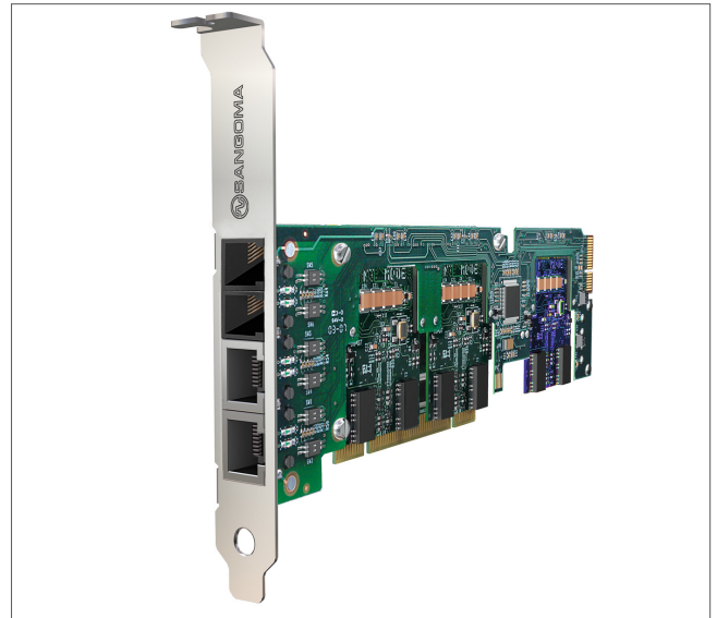
B700 with PCI interface
