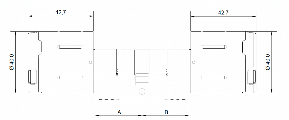
Double-Knob Cylinder
